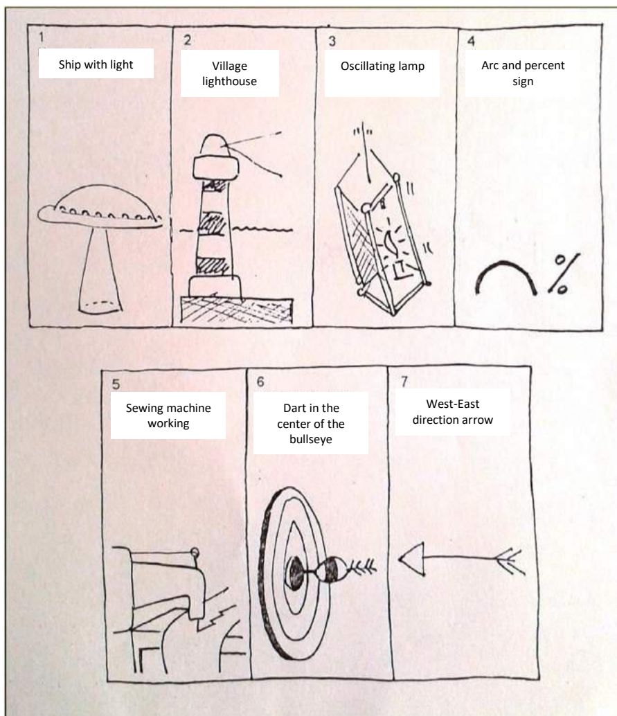
FIGURE 2. SEVEN SEQUENCES
